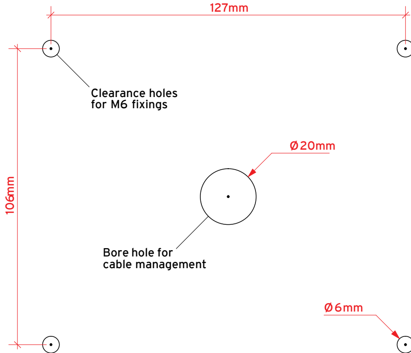
Template for optional screw mounting
