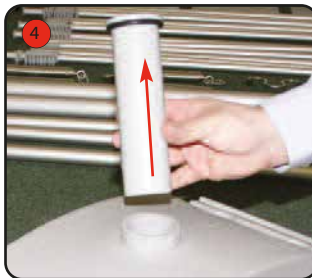
4 Remove the base tubes from the base tank. Fill each tank with water or sand, then re-fit the base tubes and fasten the screws.
